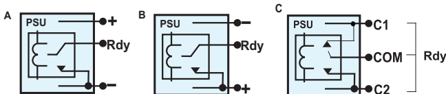
A: Non-display PSU, Rdy Internal Connection of T Type Terminal Block B: Non-display PSU, Rdy Internal Connection of E Type Terminal Block C: Display PSU, Rdy Internal Connection
