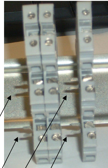
Internal Jumpers
